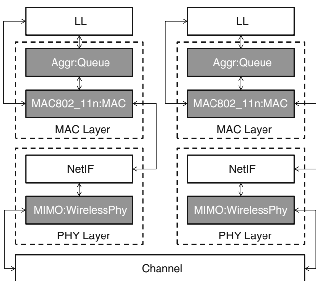
Fig. 6 NS-2 implementation
